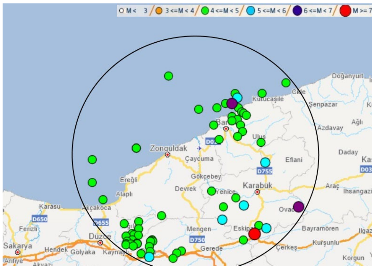
Figure 6-25: Seismicity of Within 100 km of the Aol
