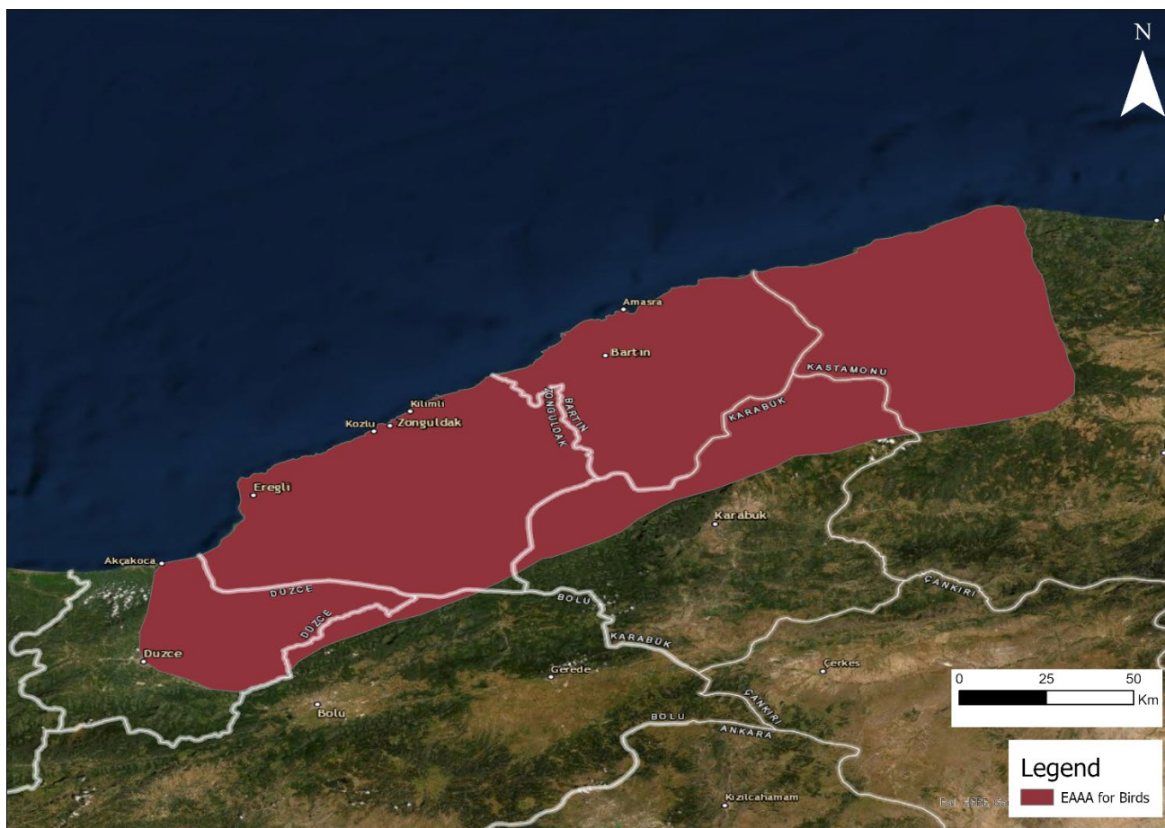
Figure 6-91: EAAA for bird species
