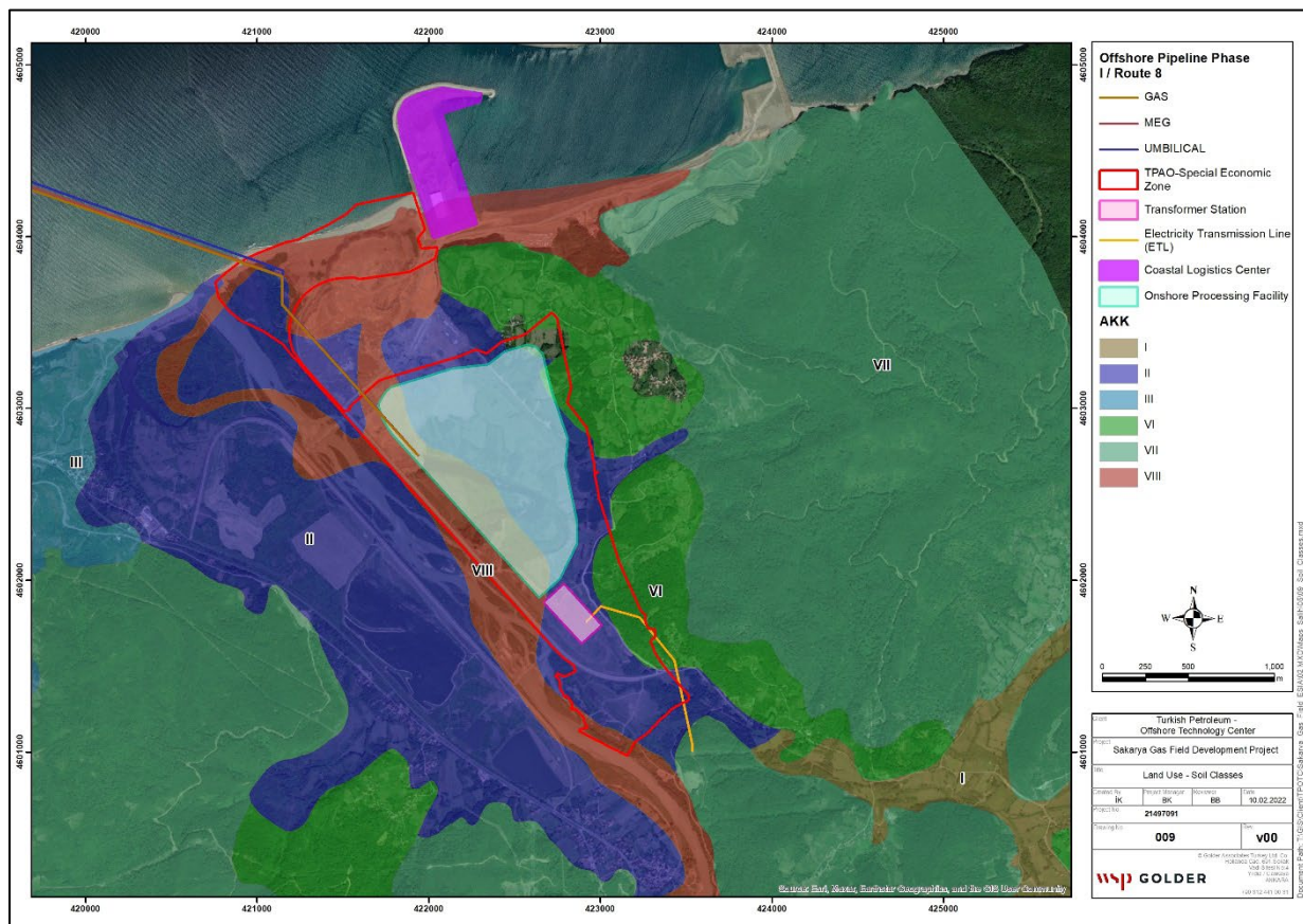
Figure 6-27: Soil Classes around Aol
