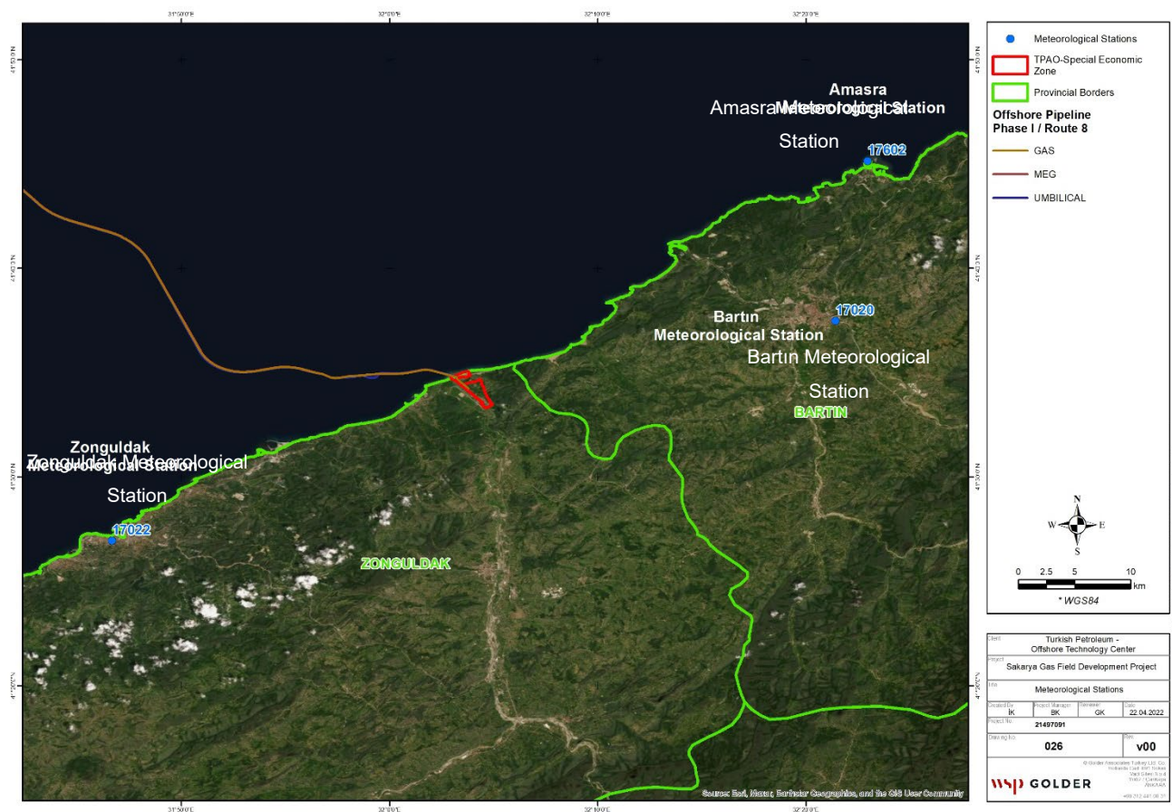
Figure 6-1: Locations of Meteorological Stations around the Project Area
